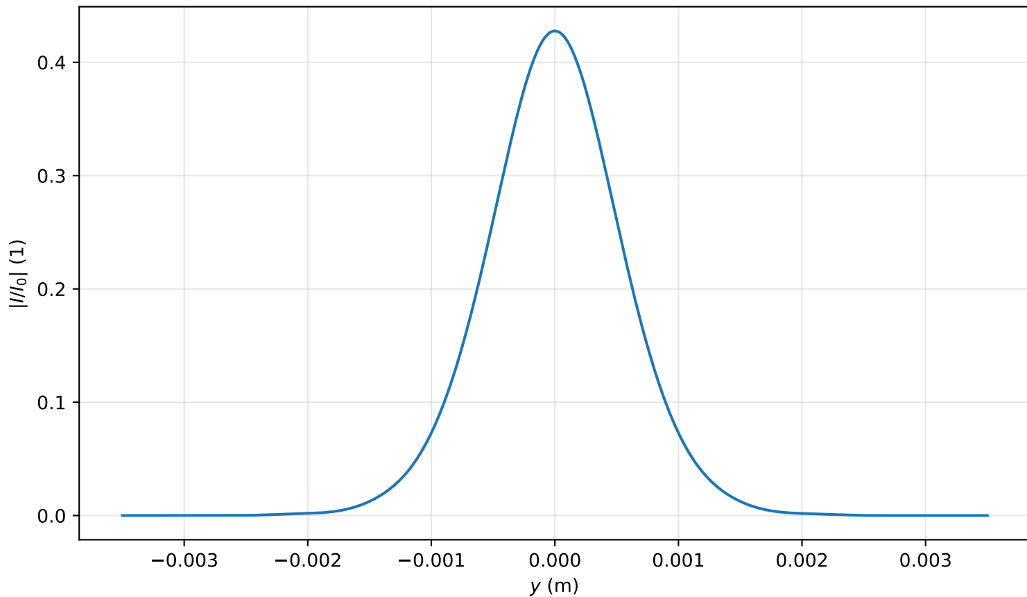
Intensity profile I(x=0, y, z=3.742)/I_0 , P_{in}=0.5P_{cr} , artificial time
